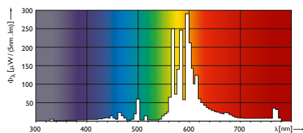
SON-T
