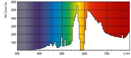
MASTER SDW-TG
